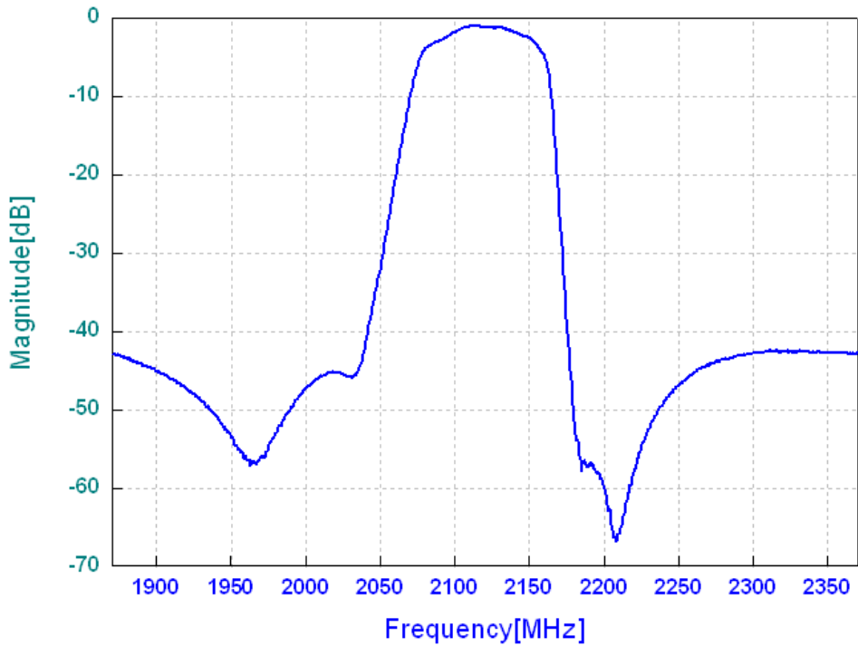
Frequency Response
